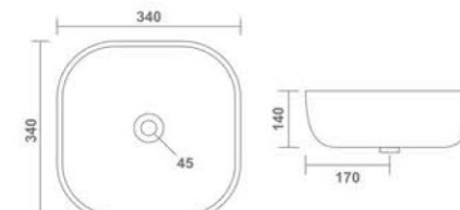
BRUCK Table Top Basin 340x340x140mm 13"x13"x5" 8.15 Kg.
