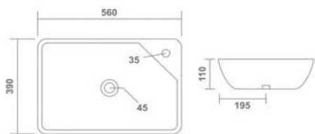
ELENA Table Top Basin 560x390x110mm 22"x15"x4" 12.85 Kg.
