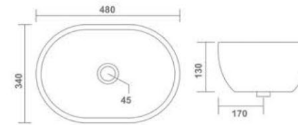
KORES Table Top Basin 480x340x130mm 19"x14"x5" 9.60 Kg.
