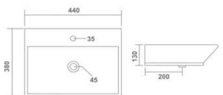
JENNY Table Top Basin 440x380x130mm 17"x15"x5" 12.10 Kg.
