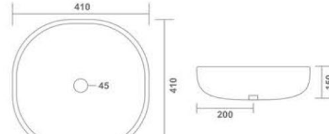
MARVEL Table Top Basin 410x410x150mm 16"x16"x6" 10.50 Kg.
