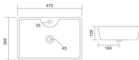
CROMA Table Top Basin 470x360x120mm 19"x14"x5" 11.30 Kg.
