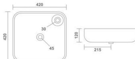
SLOG Table Top Basin 420x420x120mm 17"x17"x5" 11.80 Kg.
