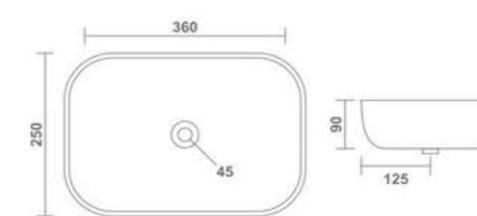
SELVI (Mini) Table Top Basin 360x250x90mm 14"x10"x4" 4.70 Kg.
