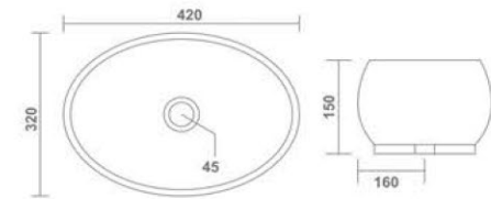
RECTA Table Top Basin 420x320x150mm 17"x13"x6" 7.55 Kg.
